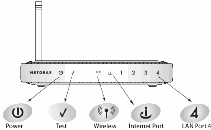
Figure 2-1: wireless router Front Panel
